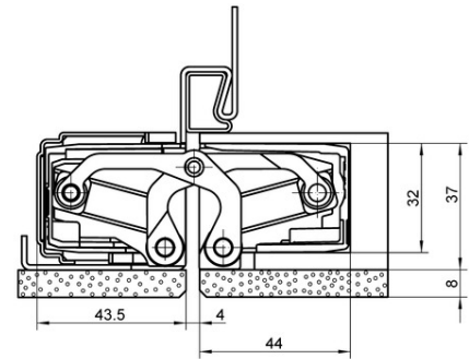
steel frame
