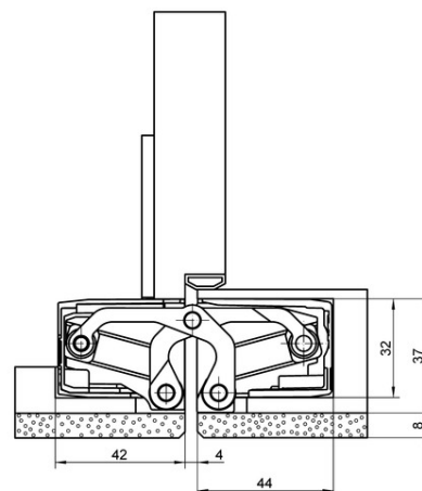
casing frame
